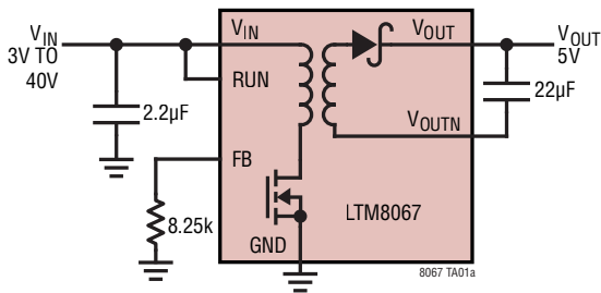
2kVAC Isolated \mu Module Regulator
